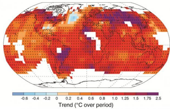
Observed change in average surface temperature 1901–2012
